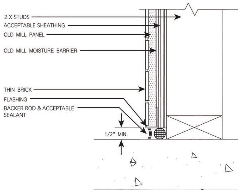
OMA-11 OLD MILL THIN BRICK SYSTEM WALL/DECK TERMINATION
