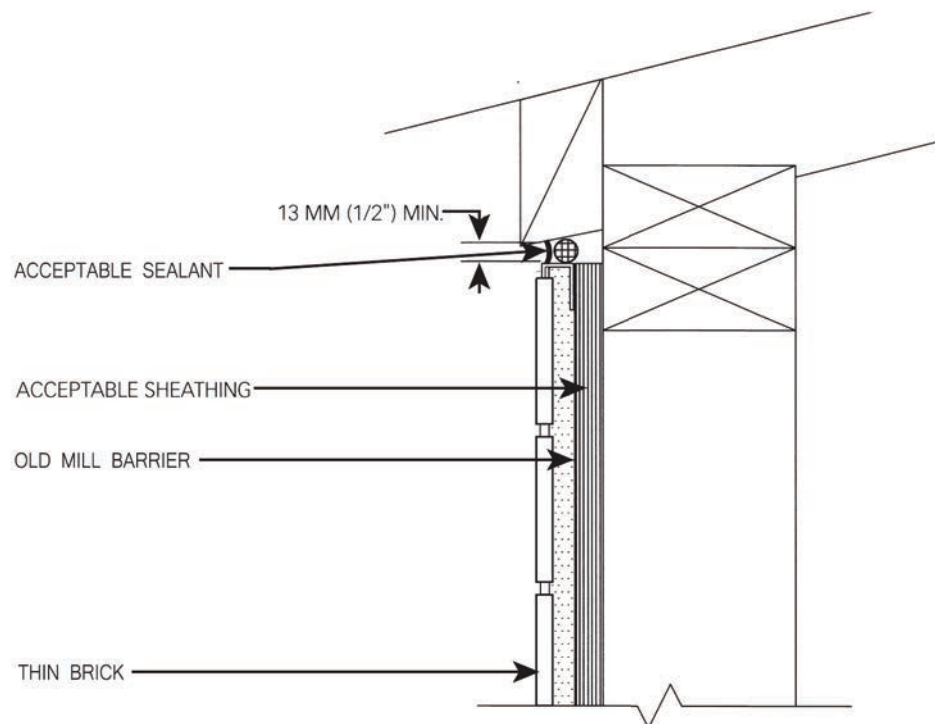
OMA-18 OLD MILL THIN BRICK SYSTEM - SOFFIT
